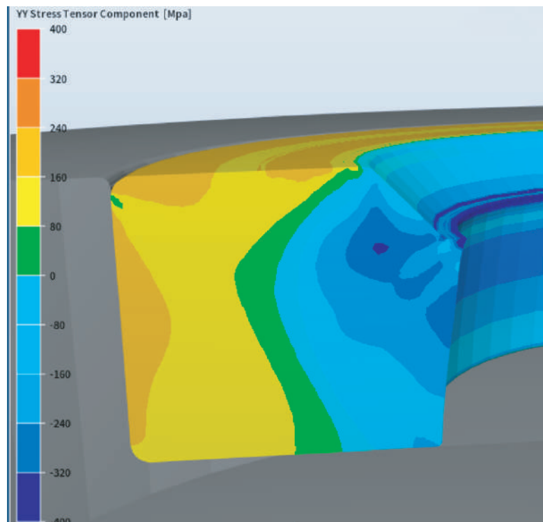
Example of part simulation
